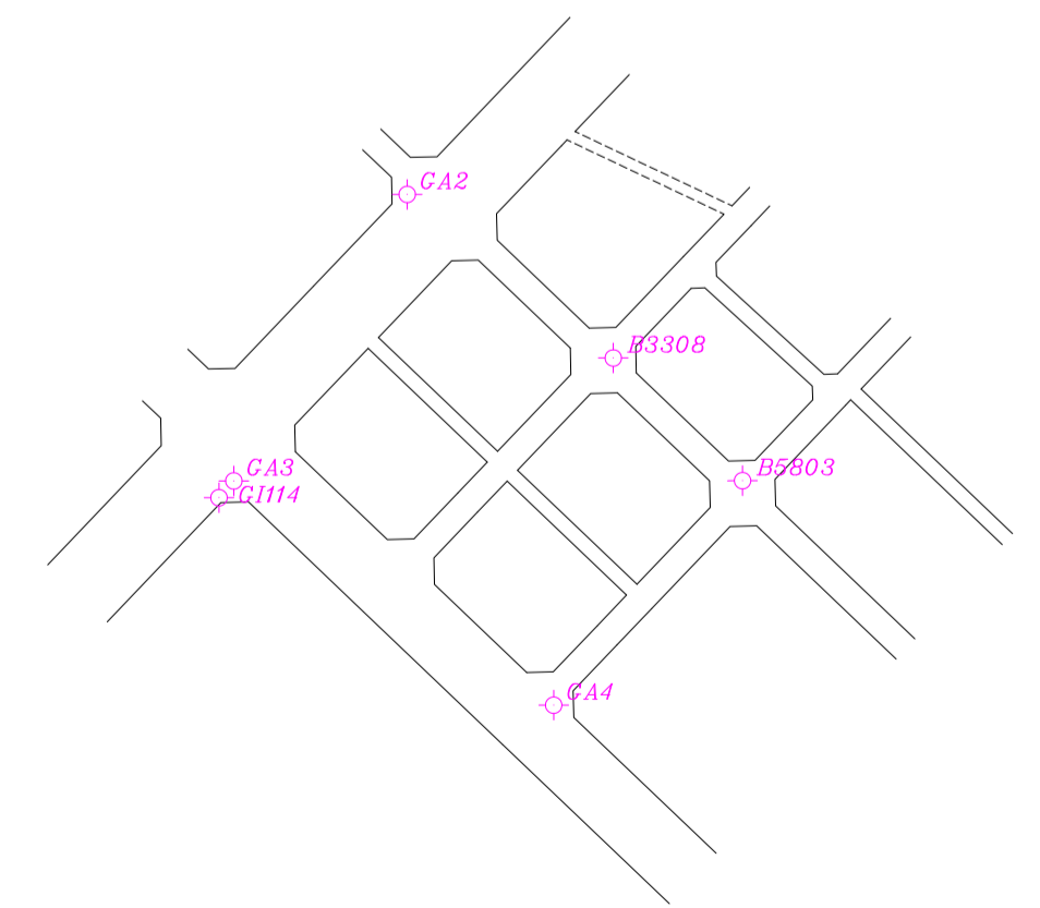
控制測量成果 SCALE=1/3000
