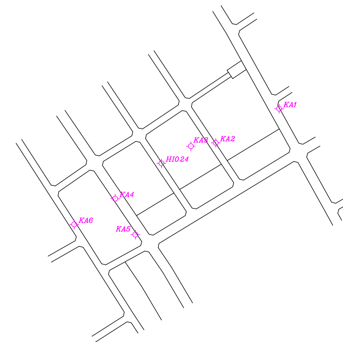
控制測量成果 SCALE=1/3000
